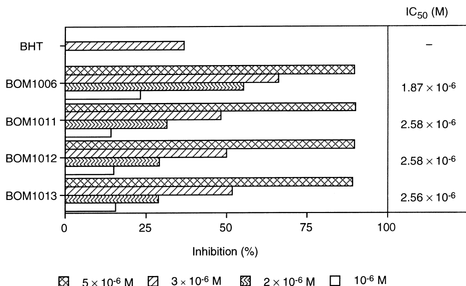
Figure 3. Effect of benzimidazole derivatives and BHT on Fe^{3+} -ADP induced NADPH dependent lipid peroxidation in rat liver microsomes. Results are the means of duplicate determinations.
