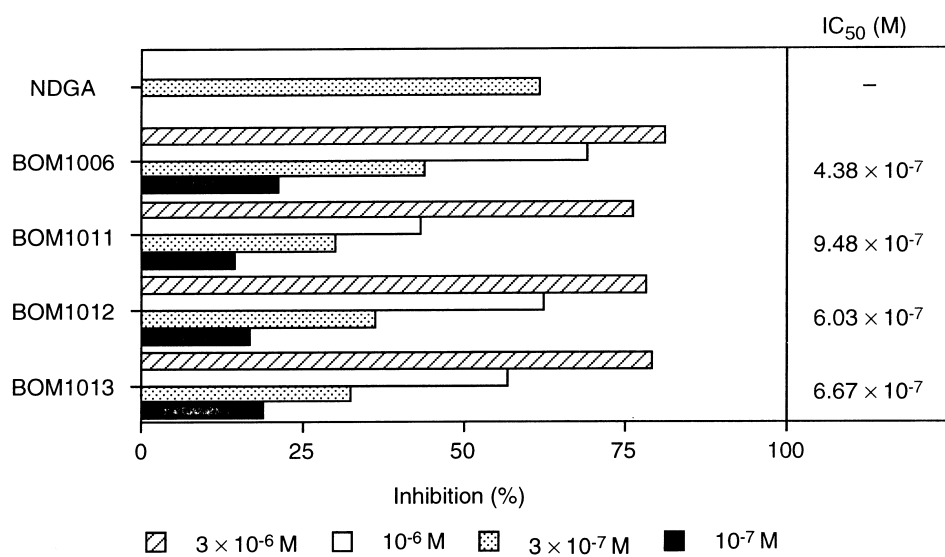
Figure 2. Effect of benzimidazole derivatives and NDGA on RBL-1 cell 5-lipoxygenase activity. Results are the means of duplicate determinations.
